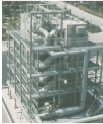
2,000 m 3 /d (0.5-mgd) vertically stacked MED plant in Japan
