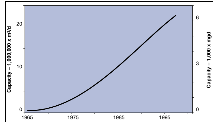
Total installed capacity of desalting facilities
