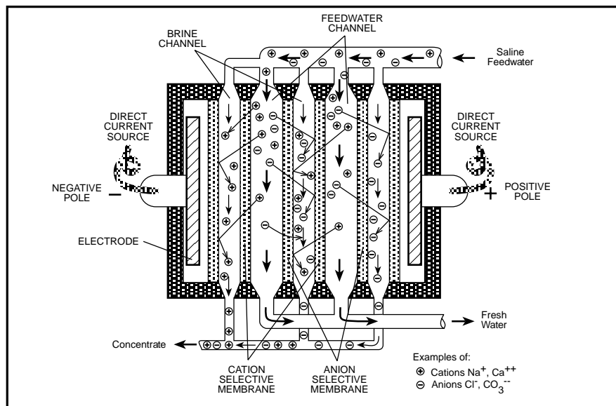
Movement of ions in the electro dialysis process
