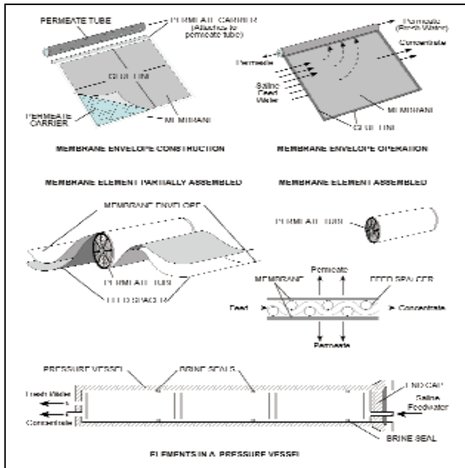
Cutaway view of a spiral membrane
