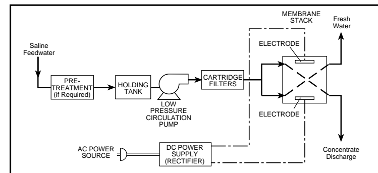
Components of an electro dialysis plant
