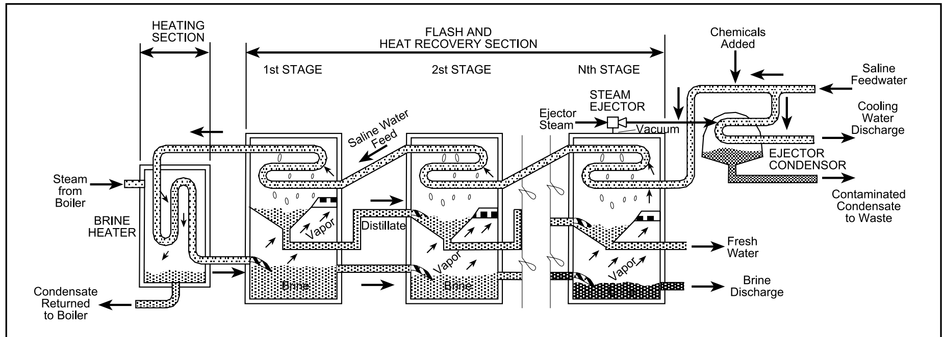
Diagram of a Multi-Stage Flash Plant
