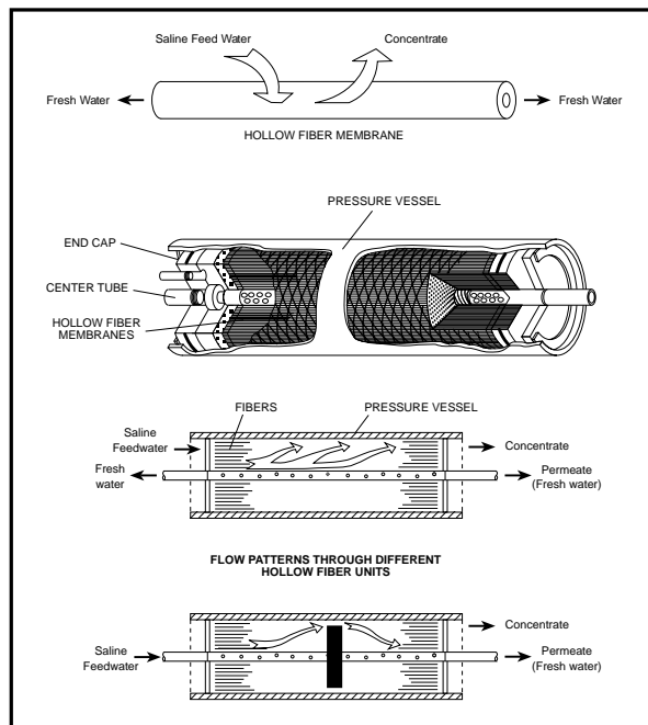
Hollow fiber membrane assembly
