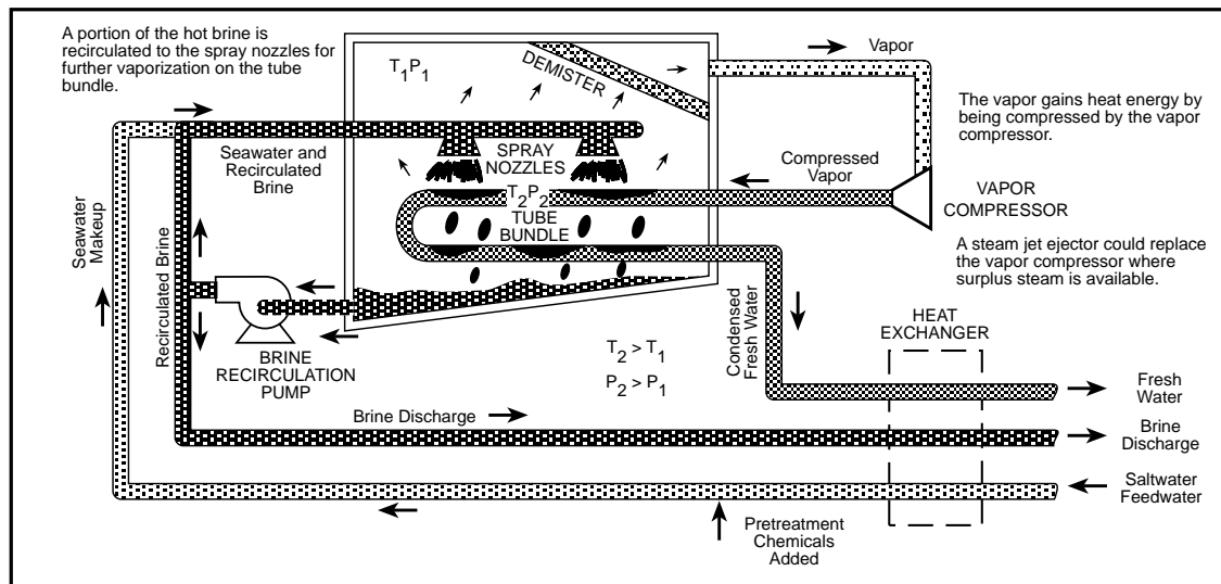
Diagram of a mechanical vapor compression unit
