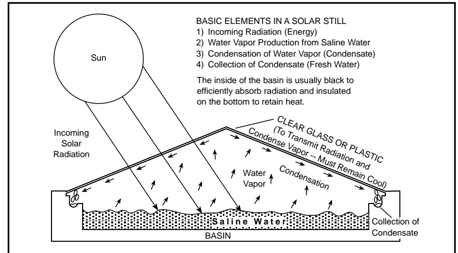
Diagram of a solar still
