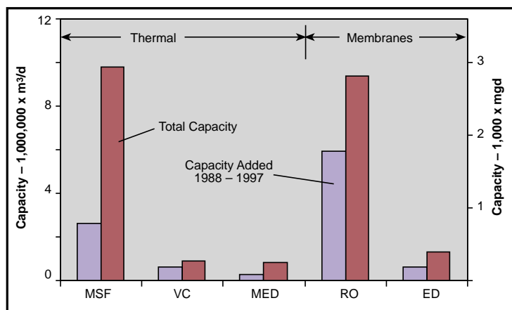
Installed capacity in the 10-year period 1987 through 1997 Source — 1998 IDA Inventory
