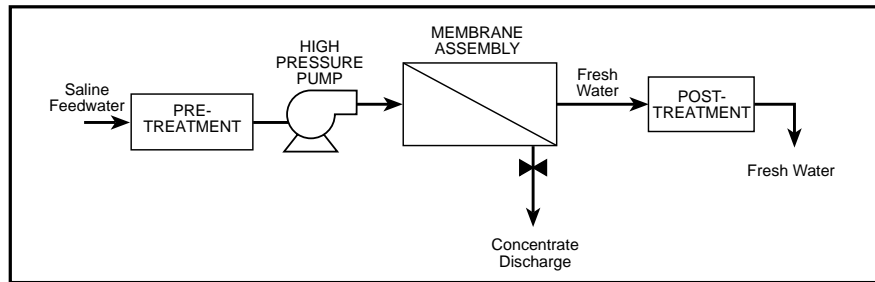
Basic components of a reverse osmosis plant
